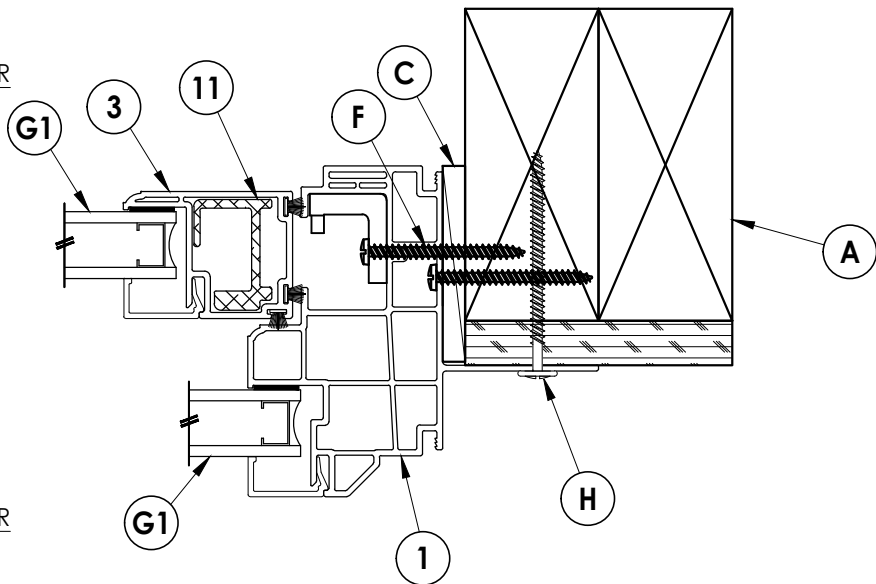
2 HORIZONTAL CROSS SECTION Shown w/ 2X Stud Construction
