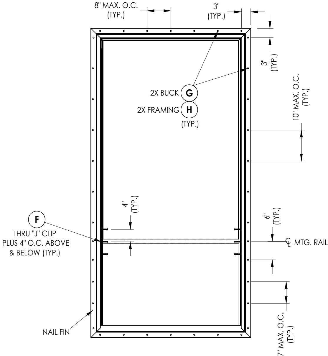
FRAME ANCHORING 48" X 96" MAX. FRAME SIZE
