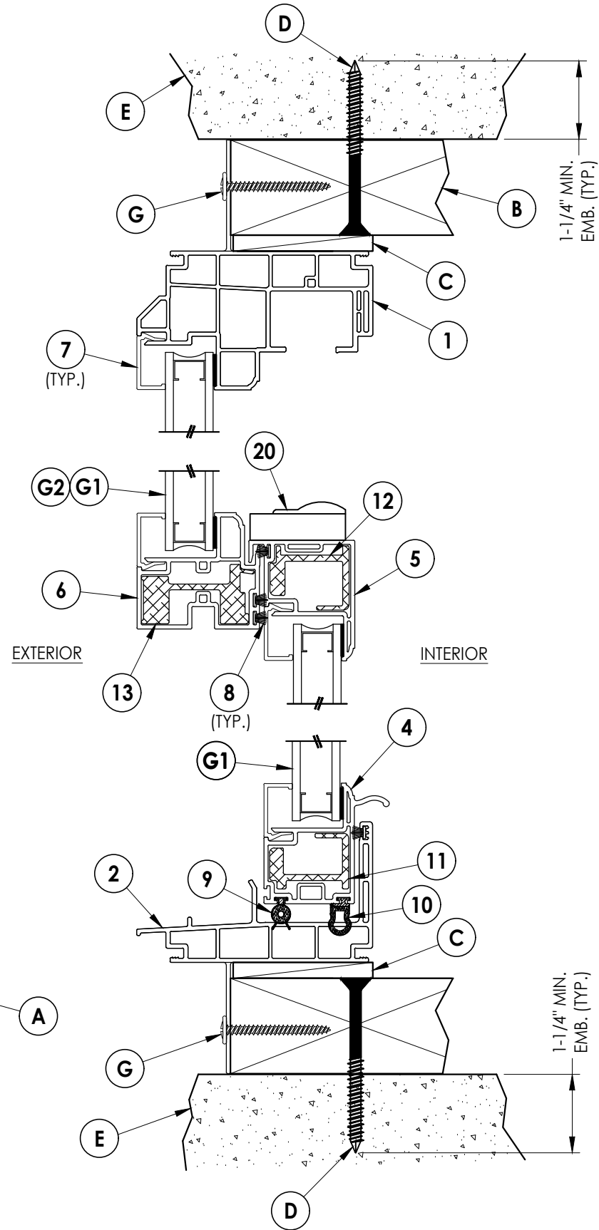
3 HORIZONTAL CROSS SECTION Shown w/ 2X buck
